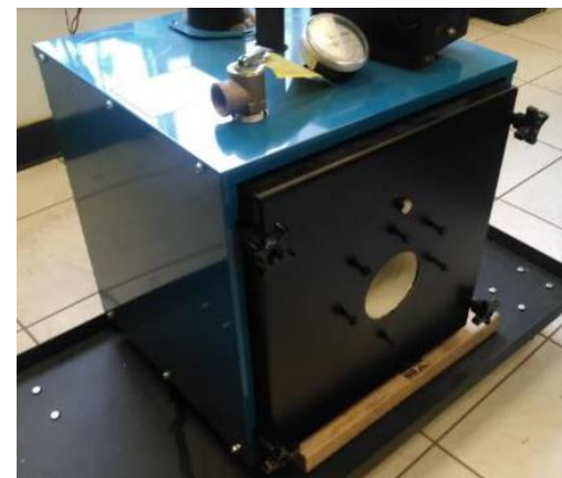
Axemann Boiler (combustion chamber)
